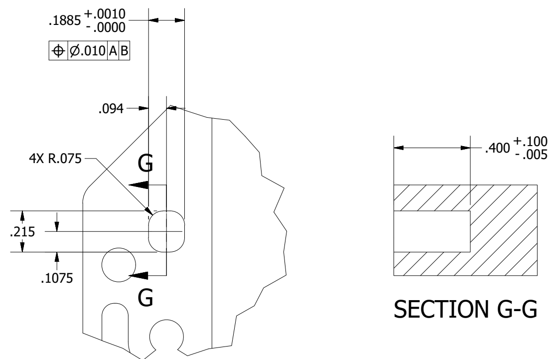
DETAIL F SLOT POCKET DIMENSIONS REPEAT OTHER SIDE
