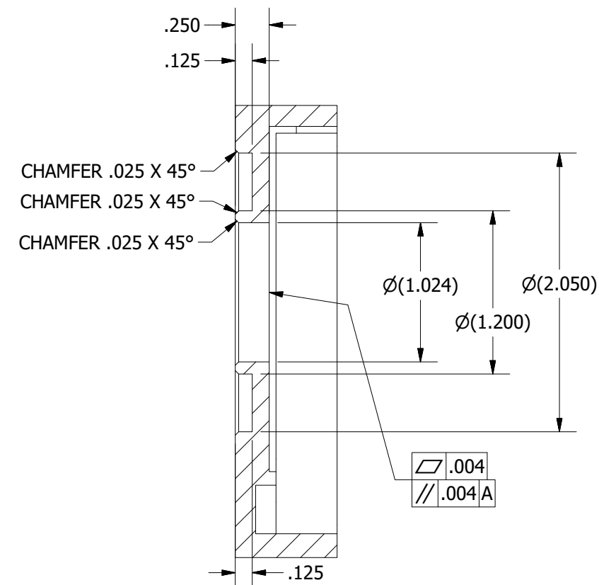
SECTION E-E
